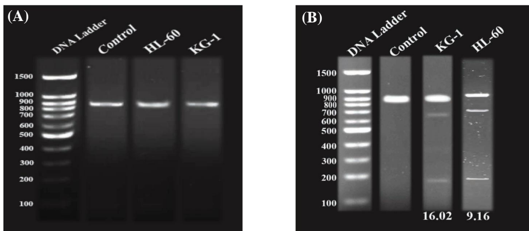
Fig. 2. CRISPR/Cas9n-mediated cleavage at BIRC5 locus in acute myelocytic leukemia cells. (A) PCR detection;(B) Surveyor assay of CRISPR/Cas9n activity in KG-1 and HL-60 cell lines. The numbers on the left represent the sizes of the DNA Ladder (bp). The numbers at the bottom of the gel indicate mutation percentages measured by band intensities.
