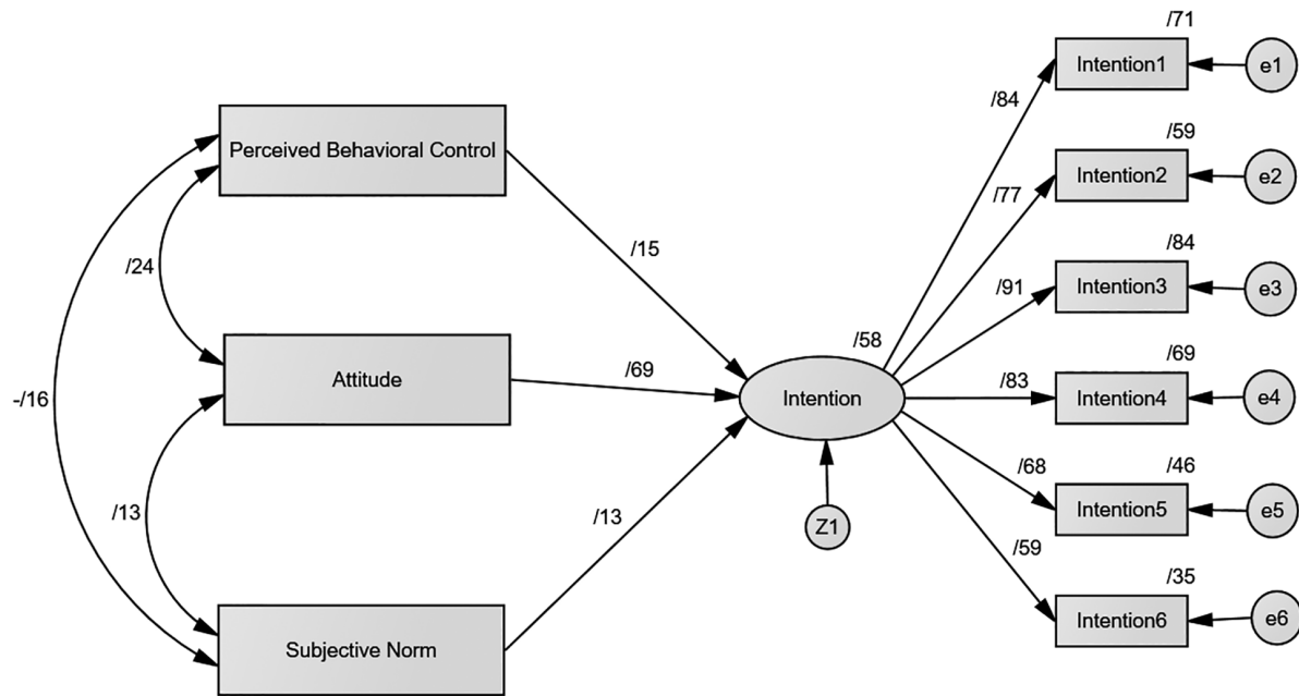
Figure 1. Path analysis of intention to file a divorce petition
