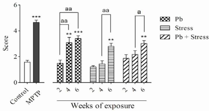
Fig. 2. Effects of 2, 4, and 6 weeks of lead exposure, restraint stress and their combination on bar test. Columns represent mean \pm SEM. Four or six weeks of lead exposure, six weeks of restraint stress, and six weeks of their co-exposure significantly ( **P < 0.01 , ***P < 0.001 ) elevated bar score compared to the control group. There are statistical differences between periods of exposures ( ^aP < 0.05 , ^{aa}P < 0.01 ). Pb, Lead; MPTP, 1-methyl-4-phenyl-1,2,3,6-tetrahydropyridine.
