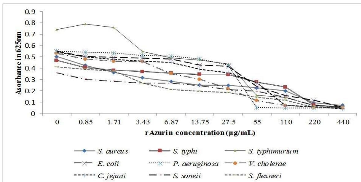
Fig. 3. The effect of rAzurin concentrations (0.85-440 µg/mL) on the growth of different bacterial species. The growth rate of bacterial species decrease by increasing of rAzurin concentrations. The absorbance of bacterial species in the presence of different concentration of rAzurin were significantly different ( p < 0.01 ) by considering MIC as breakpoint.
