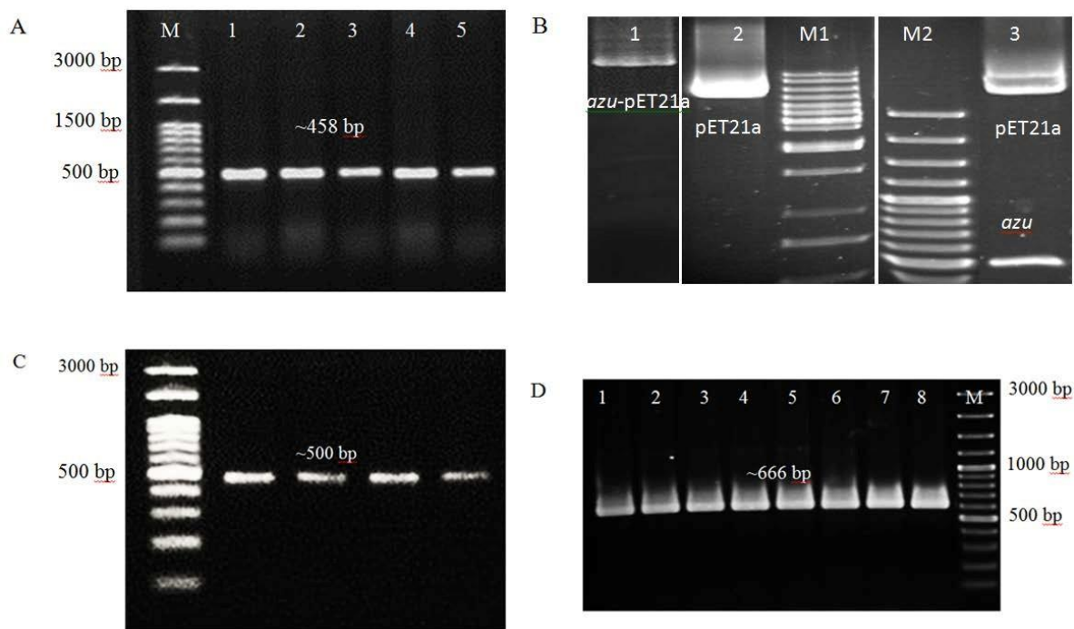
Fig. 1. (A) Agarose gel electrophoresis represents amplification of azurin gene M: DNA molecular weight 100 bp; (B) Digested and purified pET21a- azur construct and pET21a by Bam HI in line 1, and line 2, respectively, double digested of purified pET21a- azur construct by Bam HI and Nde I in line 3, M1: molecular marker 1kb, M2: molecular marker 100 bp. C, Purified azurin fragments were double digested using Nde I and Bam HI, M: molecular marker 100 bp, lines 1-4; (D) Colony PCR amplification of azurin -pET21a construct by T7 specific primers in lines 1-8, M: molecular marker 100 bp.
