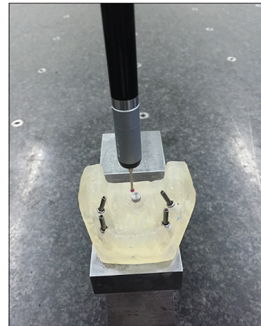
Figure 4: Using a coordinate measuring machine for measuring position and direction of implants.
