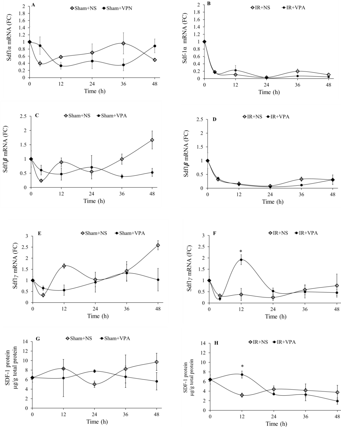
Fig. 3. VPA restores the down-regulation of SDF-1 following kidney ischemia. The expression of Sdf-1 alpha mRNA is measured over time in (A) sham + NS and sham + VPA groups as well as (B) IR + NS and IR+VPA groups. Also, (C and D) Sdf-1 beta mRNA is measured in sham + NS and sham + VPA groups and IR + NS and IR + VPA groups, respectively. In addition, (E and F) the expression of Sdf-1 gamma mRNA is quantified in sham + NS and sham + VPA groups as well as IR + NS and IR + VPA groups, respectively. Similarly, (G and H) SDF-1 is measured at the protein level in in sham + NS and sham + VPA groups as well as IR+NS and IR+VPA groups, respectively. * P < 0.05 indicates statistically significant differences between the groups at the same time points. IR, Ischemia reperfusion; NS, normal saline; SDF-1, stromal derived factor-1; VPA, valproic acid.
