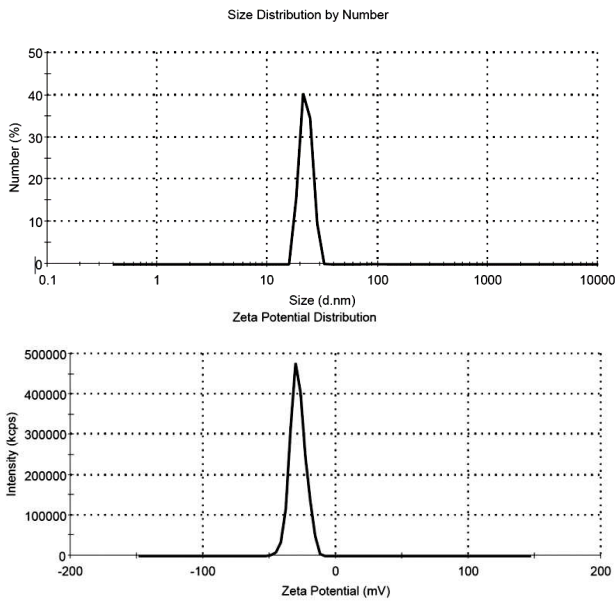
Figure 4. Dynamic light scattering measurements (DLS) of GNPs (peak: 22.4 nm) and Zeta potential measurements of GNPs (peak: -28.5 mV).
