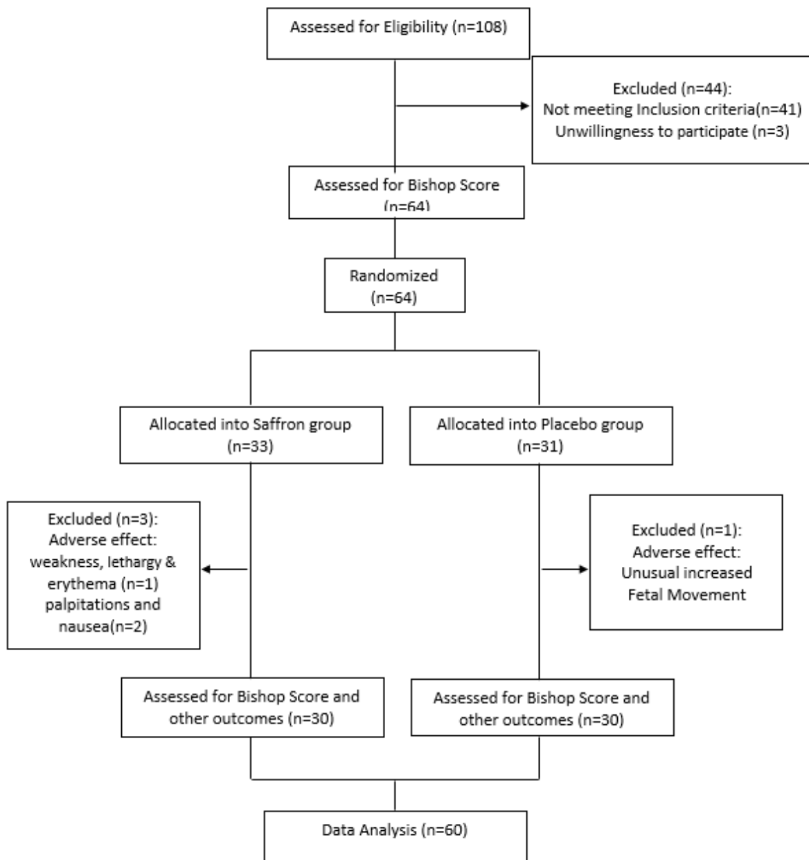
Fig.1: Study Flowchart.
